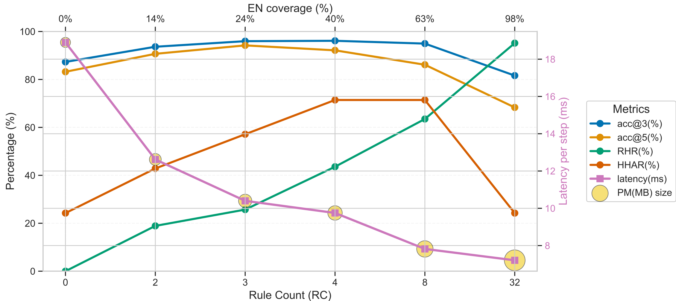
Speed–accuracy–memory trade-off (Car_Following)
